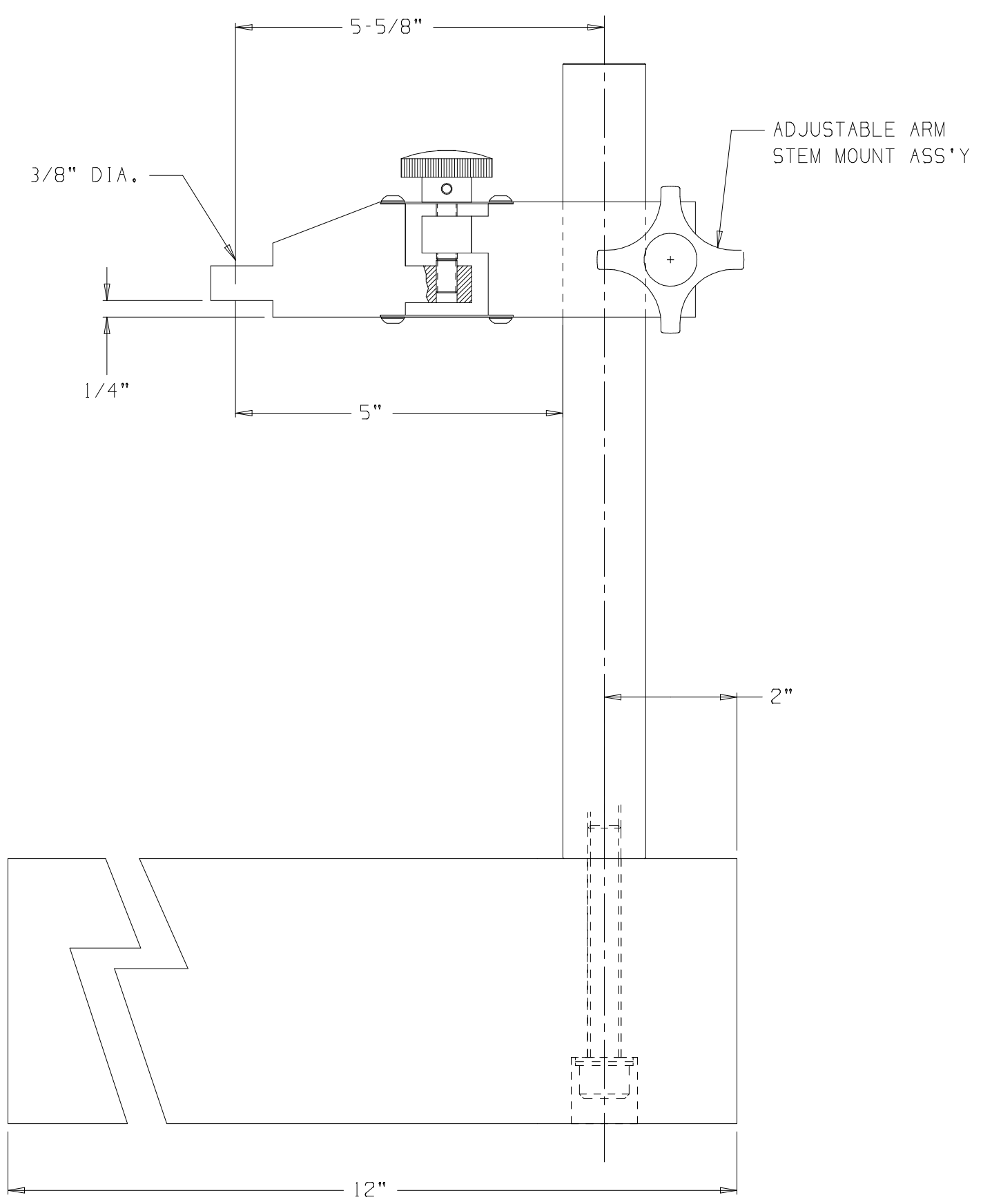
(61812-1S) GRANITE BASE 18" X 12" X 4" W/ADJUSTABLE ARM, STEM MOUNT
