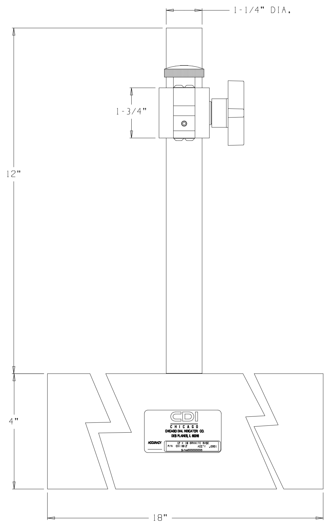
(61812-1S) GRANITE BASE 18" X 12" X 4" W/ADJUSTABLE ARM, STEM MOUNT
