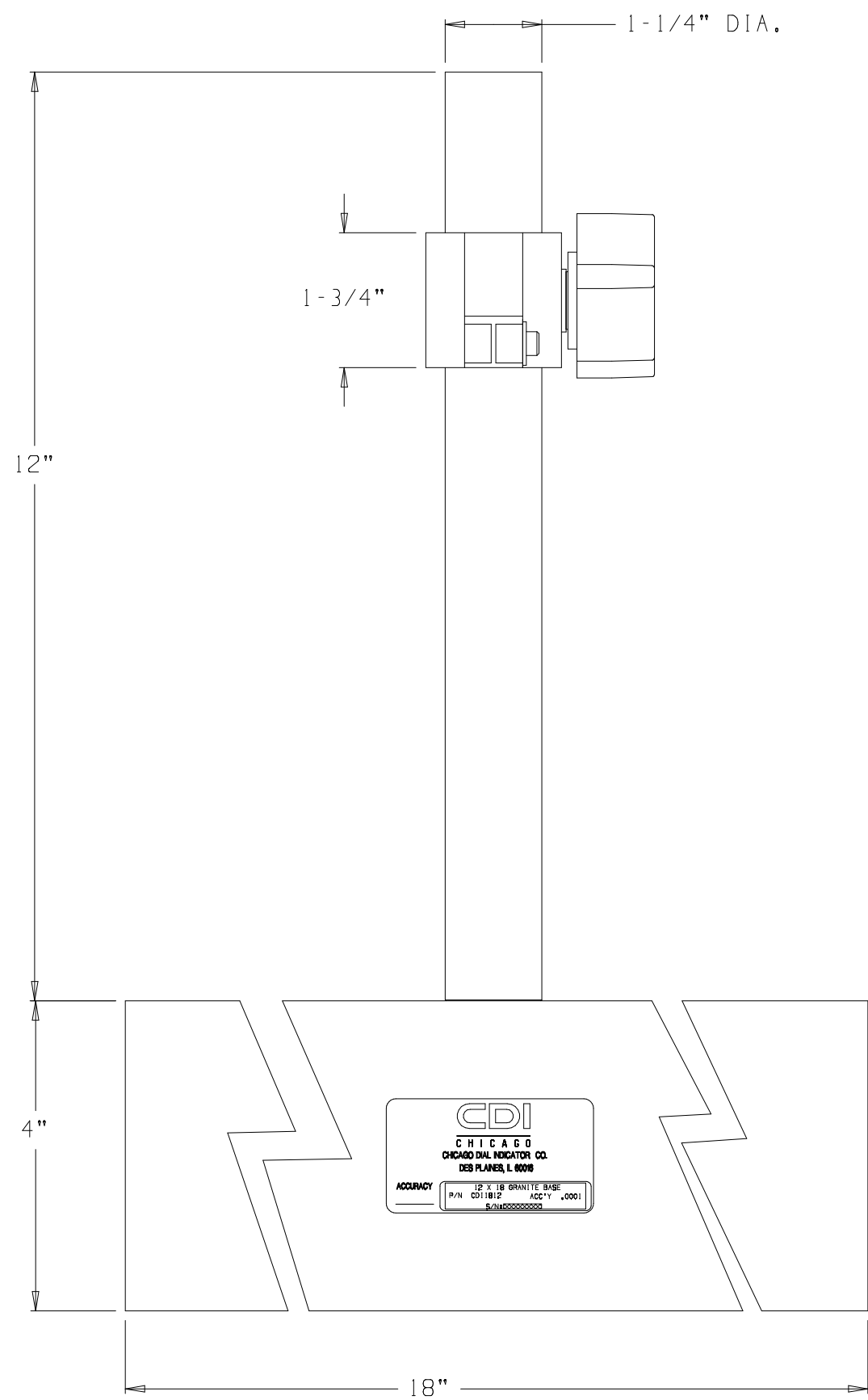
(61812-1RS) GRANITE BASE 18" X 12" X 4" W/RIGID ARM, STEM MOUNT
