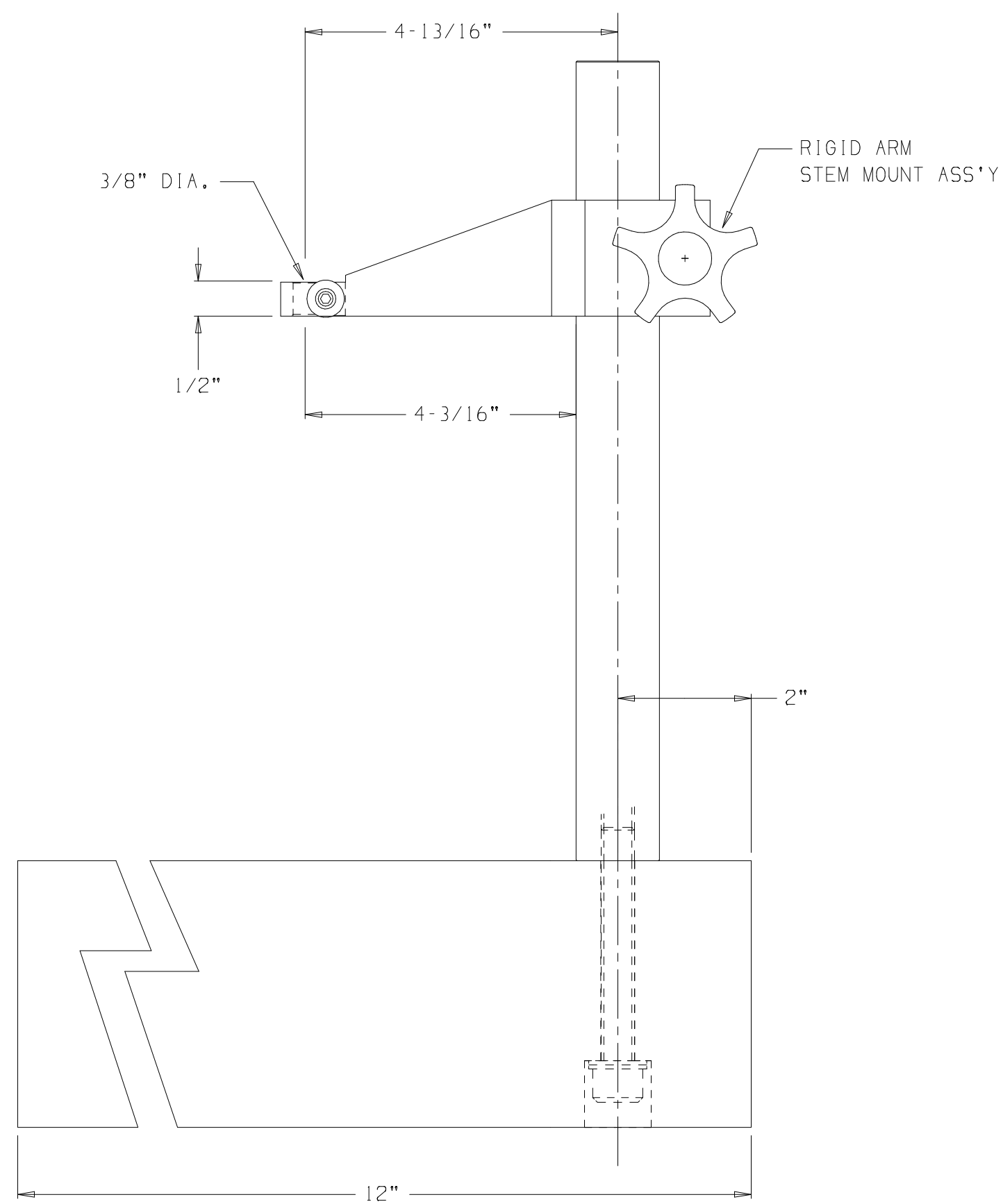
(61812-1RS) GRANITE BASE 18" X 12" X 4" W/RIGID ARM, STEM MOUNT
