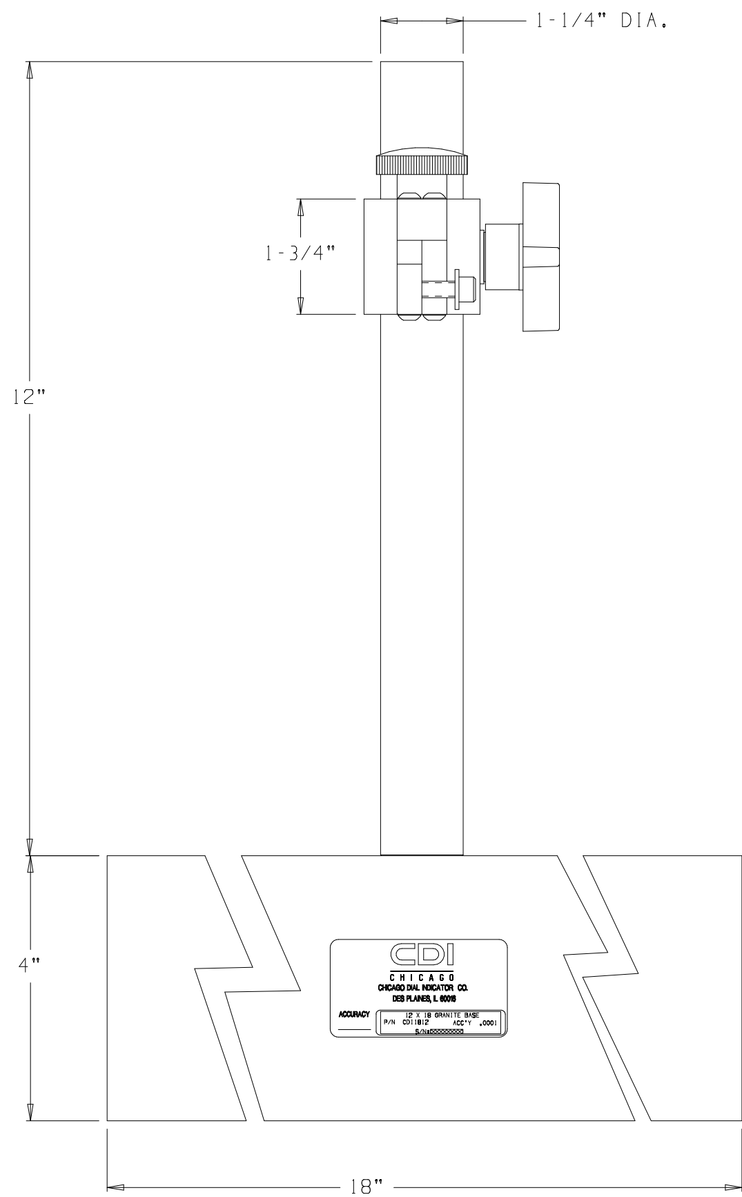
(61812-1) GRANITE BASE 18" X 12" X 4" W/ADJUSTABLE ARM, LUG MOUNT
