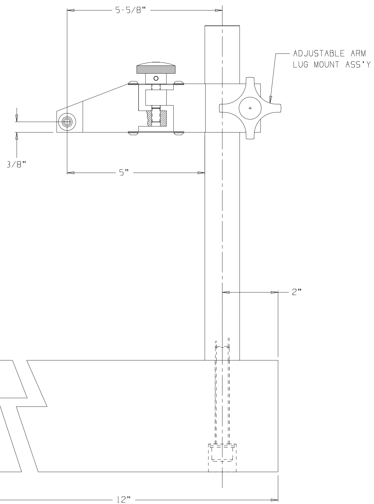
(61812-1) GRANITE BASE 18" X 12" X 4" W/ADJUSTABLE ARM, LUG MOUNT
