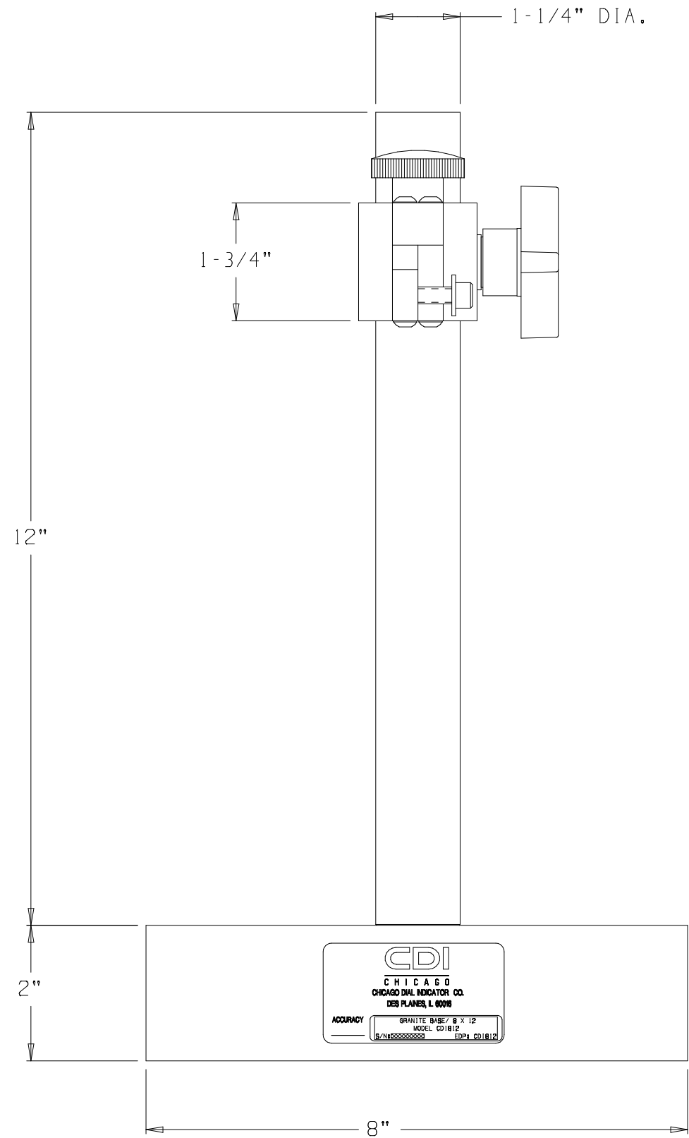
(60812-1) GRANITE BASE 8" X 12" X 2" W/ADJUSTABLE ARM, LUG MOUNT
