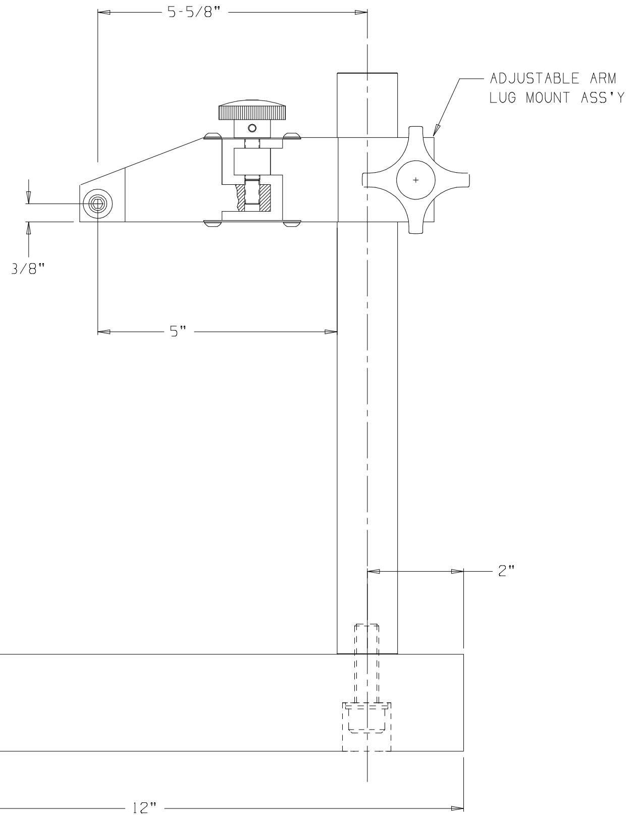
(60812-1) GRANITE BASE 8" X 12" X 2" W/ADJUSTABLE ARM, LUG MOUNT
