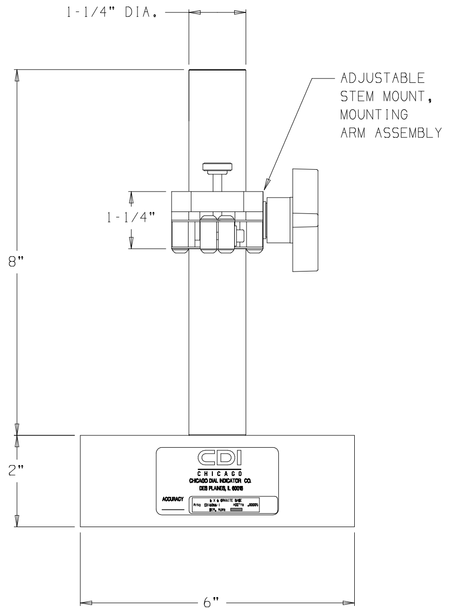
(6066-20S) GRANITE BASE 6" X 6" X 2" W/ADJUSTABLE ARM STEM MOUNT
