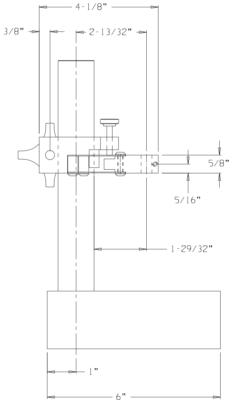
(6066-20S) GRANITE BASE 6" X 6" X 2" W/ADJUSTABLE ARM STEM MOUNT
