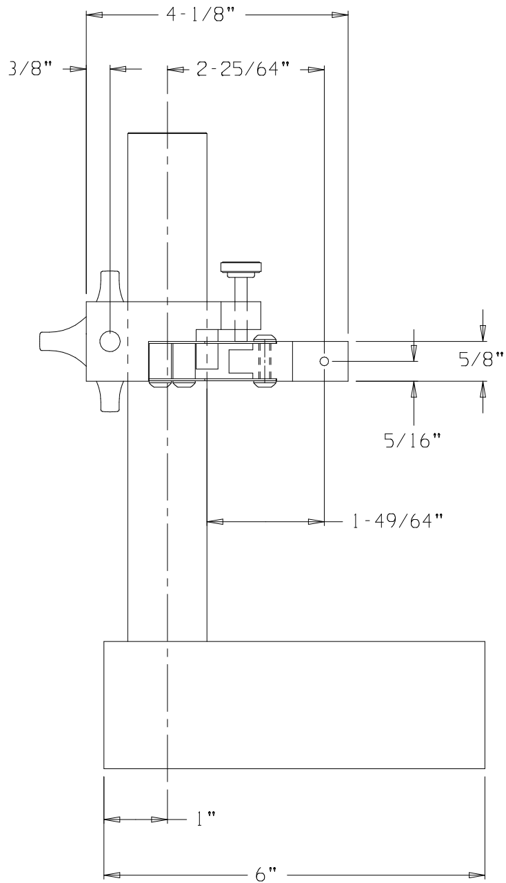
(6066-20) GRANITE BASE 6" X 6" X 2" W/ADJUSTABLE ARM LUG MOUNT
