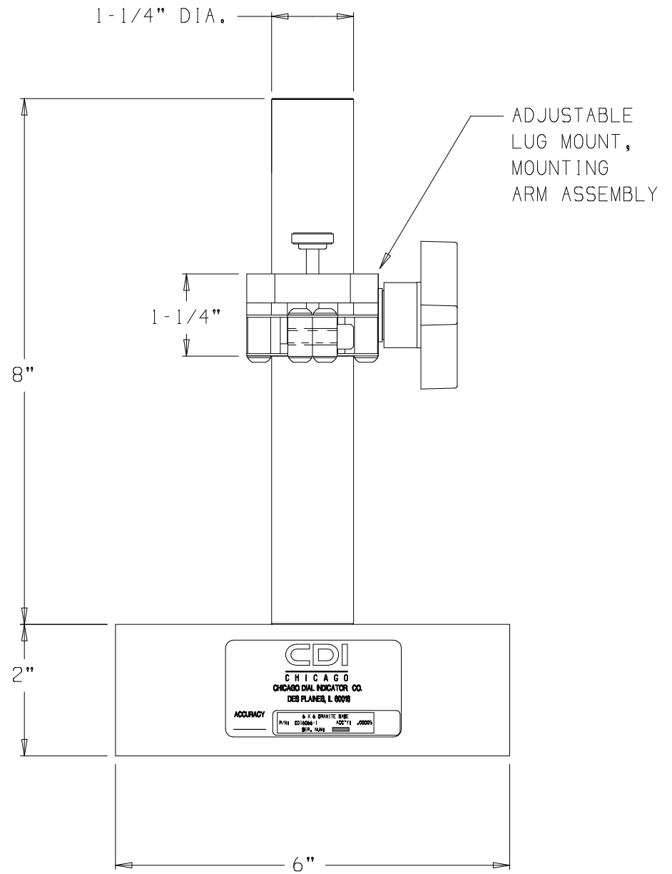
(6066-20) GRANITE BASE 6" X 6" X 2" W/ADJUSTABLE ARM LUG MOUNT
